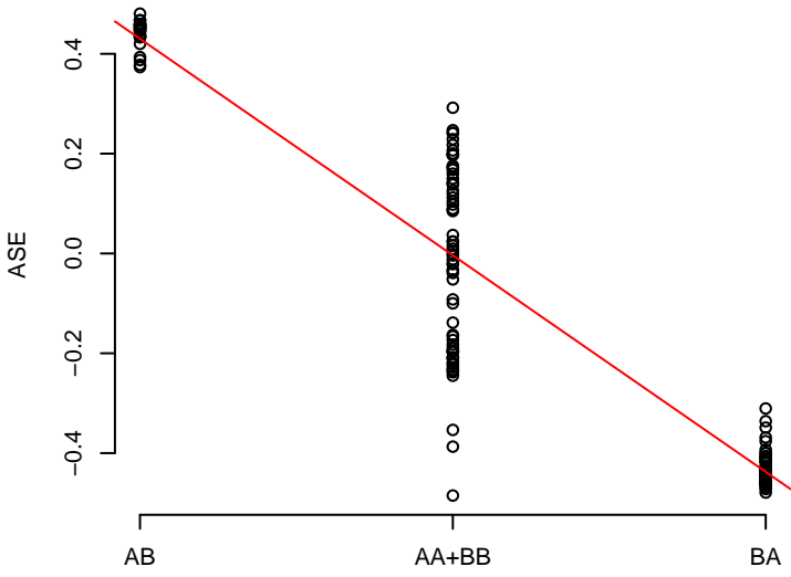
25 rs657152
