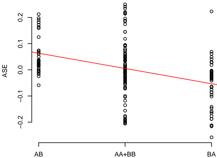
19 rs1299548
