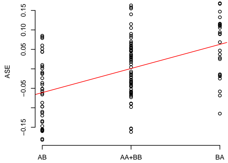
8 rs2303393
