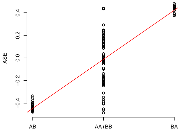
24 rs687621
