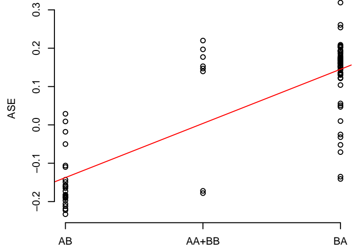
34 rs1153862
