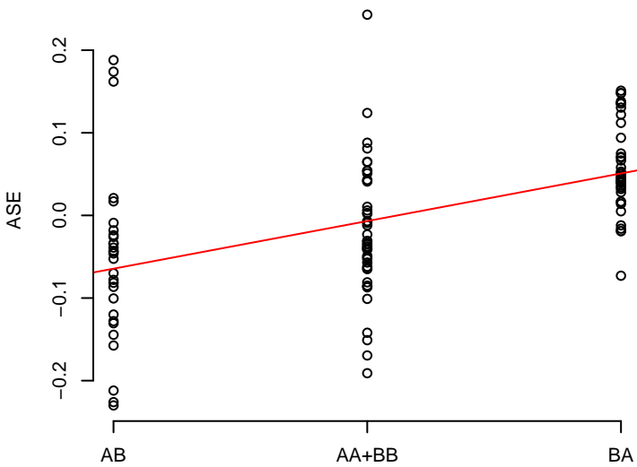
11 rs6922111
