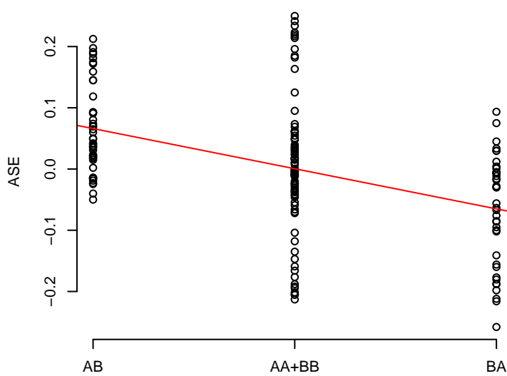
18 rs10259085
