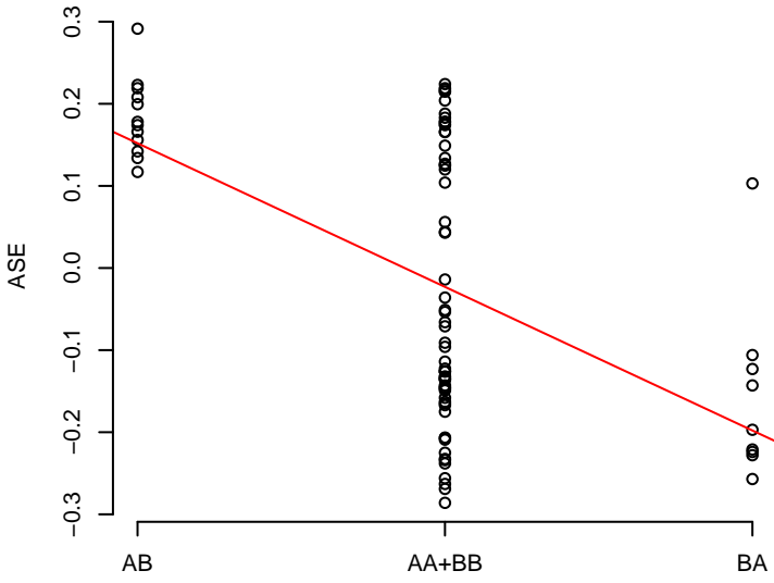
33 rs7896729
