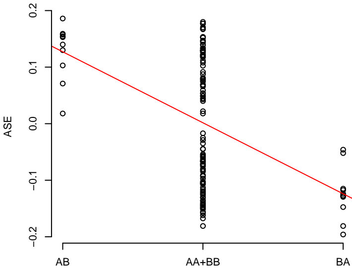
1 rs2501276
