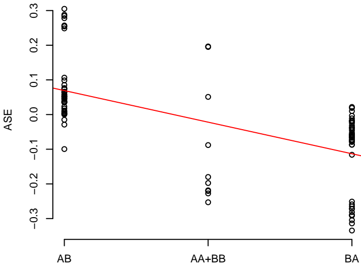
3 rs6663565
