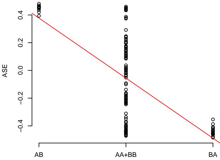
29 rs507666
