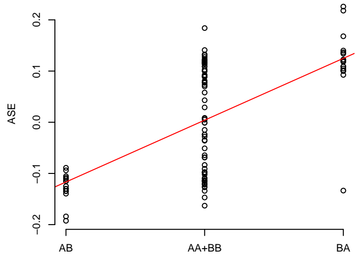
10 rs7686660
