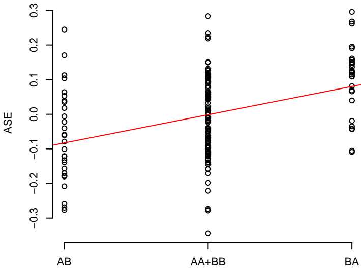
13 rs7739434
