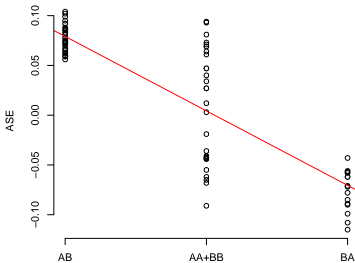
16 rs4928431
