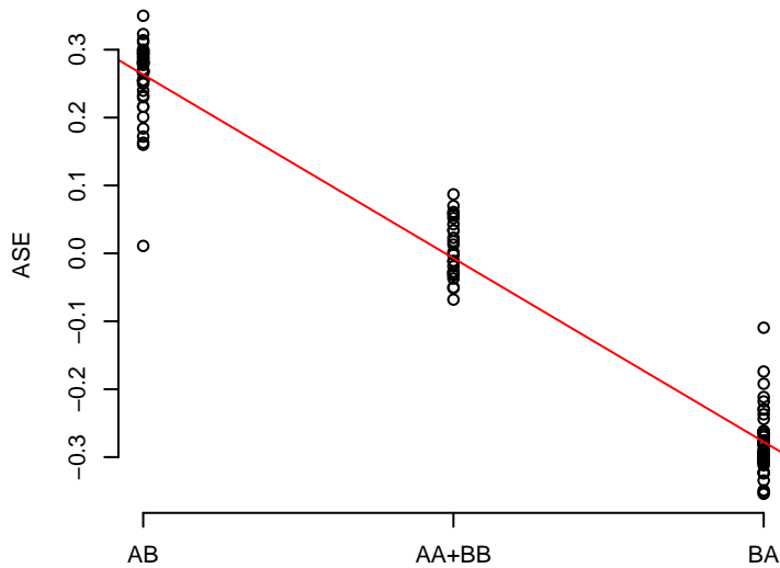
20 rs13278062
