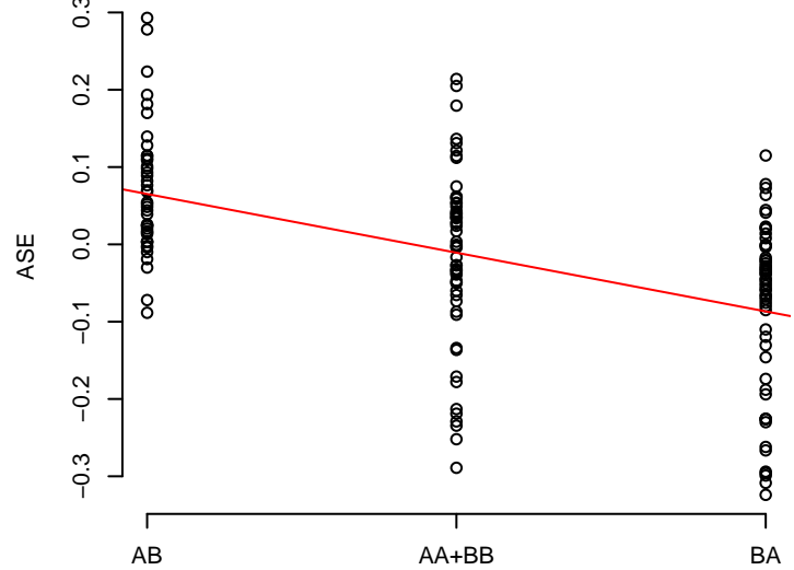
12 rs3893464
