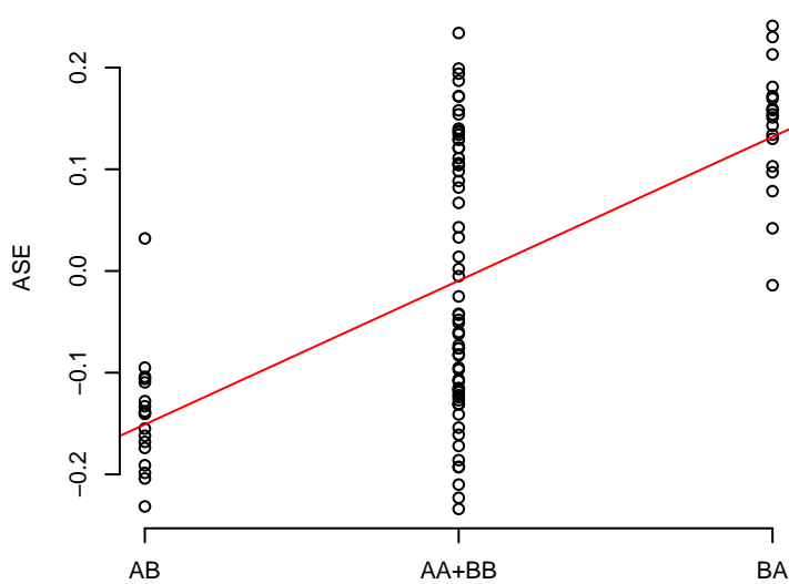
14 rs13214831
