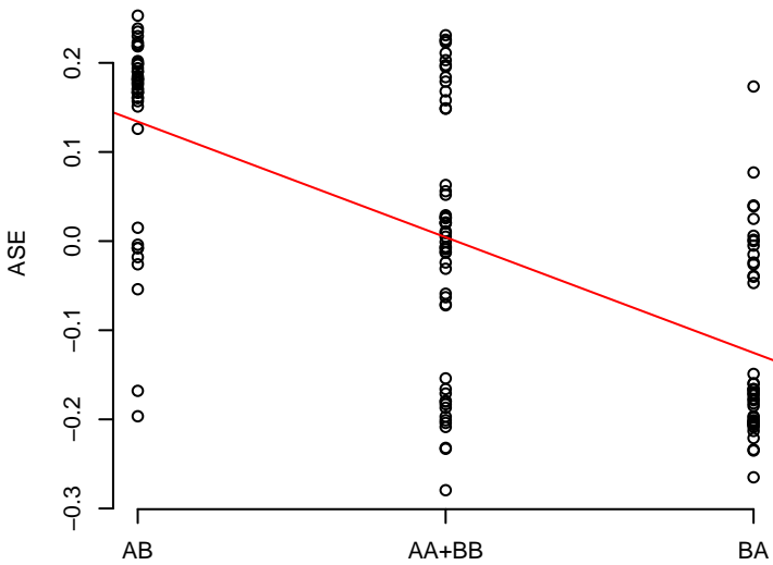
23 rs3761847
