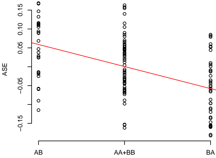
7 rs6710518
