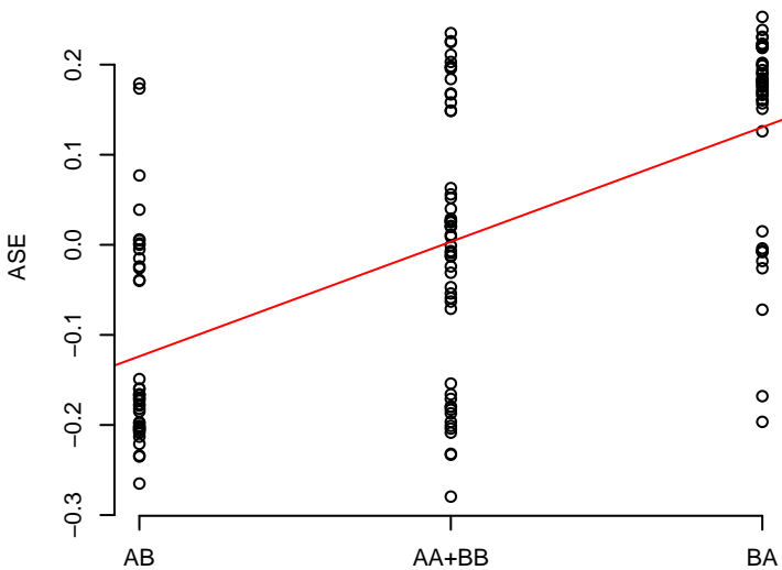
21 rs1953126
