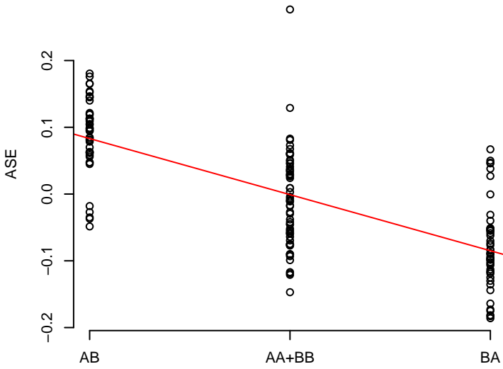
9 rs12638253
