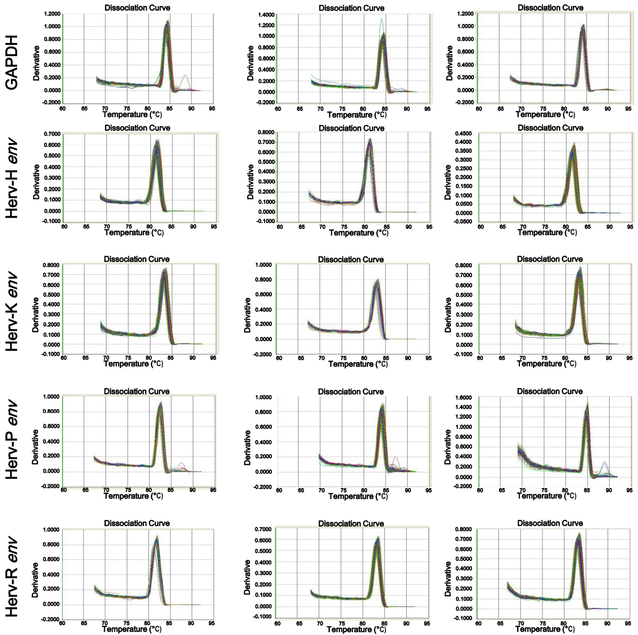
Figure S1. Comparative melt curves of all amplified products.
