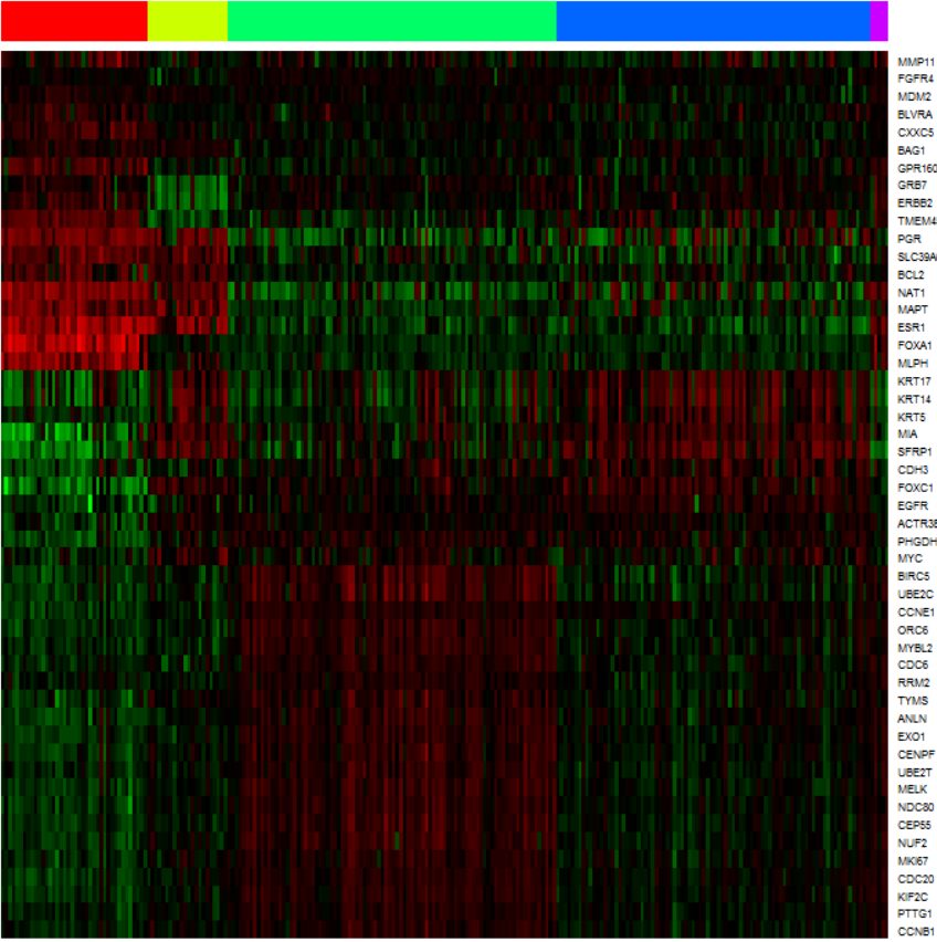
Figure S1. Heatmap visualizing the PAM50 genes on the Agilent dataset. Color coding represents PAM50 subtype classification results: Red: Basal; Yellow: HER2-enriched; Green: Luminal-A; Blue: Luminal-B; Purple: Normal-like.
