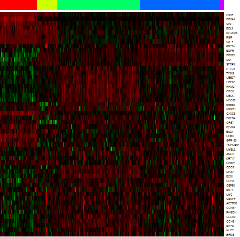
Figure S2. Heatmap visualizing the PAM50 genes on the 29K unadjusted dataset. Color coding represents PAM50 subtype classification results: Red: Basal; Yellow: HER2-enriched; Green: Luminal-A; Blue: Luminal-B; Purple: Normal-like.
