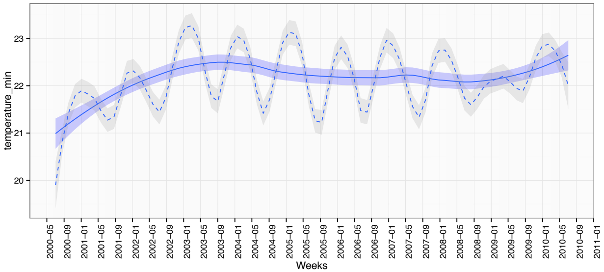
Figure S6: Seasonal (a) and long-term (b) trends of minimum temperature in Iquitos, Peru. In (a), annual trimesters (demarcated by dashed vertical lines) and the dengue season (red shaded area) are indicated. The blue line is the loess smoothed response with standard error, \alpha = 0.5 . In (b), solid line is the loess smoothed response with standard error ( \alpha = 0.5 , blue envelope). The dashed line is for \alpha = 0.1 with standard error (grey envelope, See Methods).
