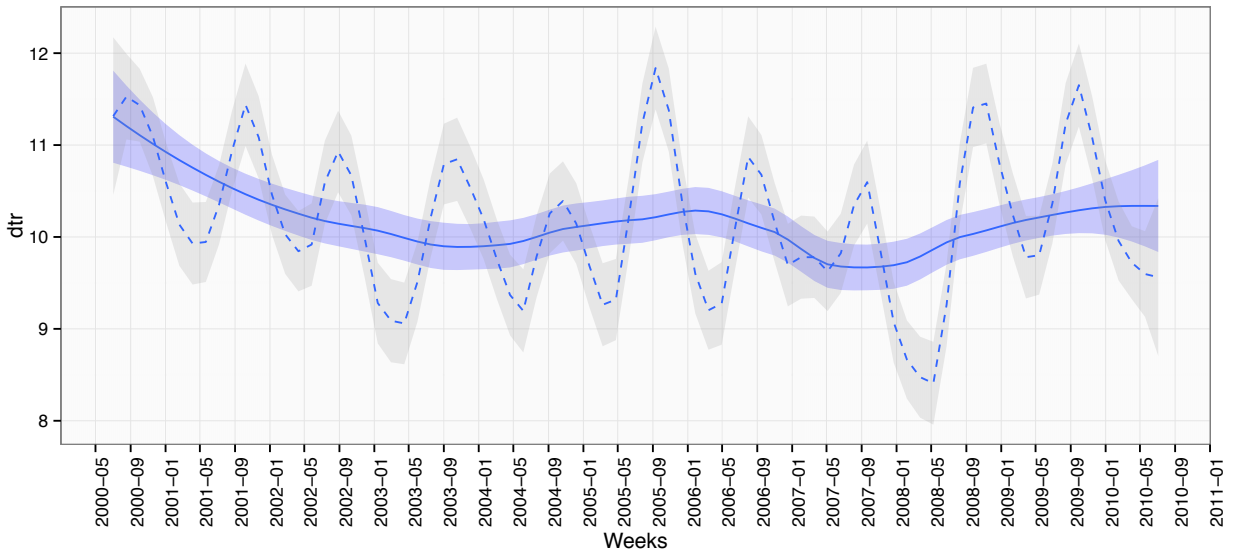
Figure S10: Seasonal (a) and long-term (b) trends of DTR in Iquitos, Peru. In (a), annual trimesters (demarcated by dashed vertical lines) and the dengue season (red shaded area) are indicated. The blue line is the loess smoothed response with standard error, \alpha = 0.5 . In (b), solid line is the loess smoothed response with standard error ( \alpha = 0.5 , blue envelope). The dashed line is for \alpha = 0.1 with standard error (grey envelope, See Methods).
