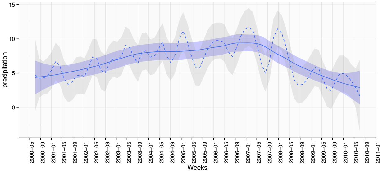
Figure S12: Seasonal (a) and long-term (b) trends of total weekly precipitation (cm) in Iquitos, Peru. In (a), annual trimesters (demarcated by dashed vertical lines) and the dengue season (red shaded area) are indicated. The blue line is the loess smoothed response with standard error, \alpha = 0.5 . In (b), solid line is the loess smoothed response with standard error ( \alpha = 0.5 , blue envelope). The dashed line is for \alpha = 0.1 with standard error (grey envelope, See Methods).
