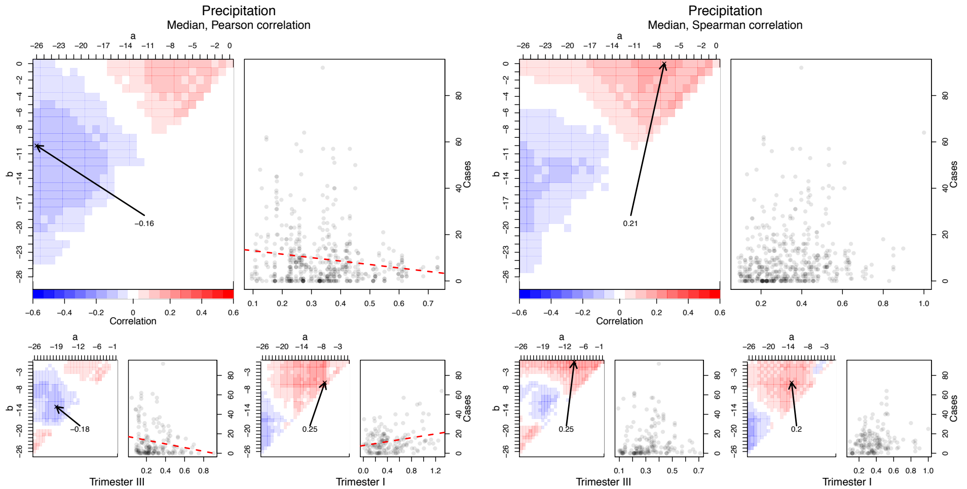
Figure S13: CCM and scatterplot at lag of highest |r| in Spearman and Pearson correlations for the whole year (large panels) and trimesters I and III.
