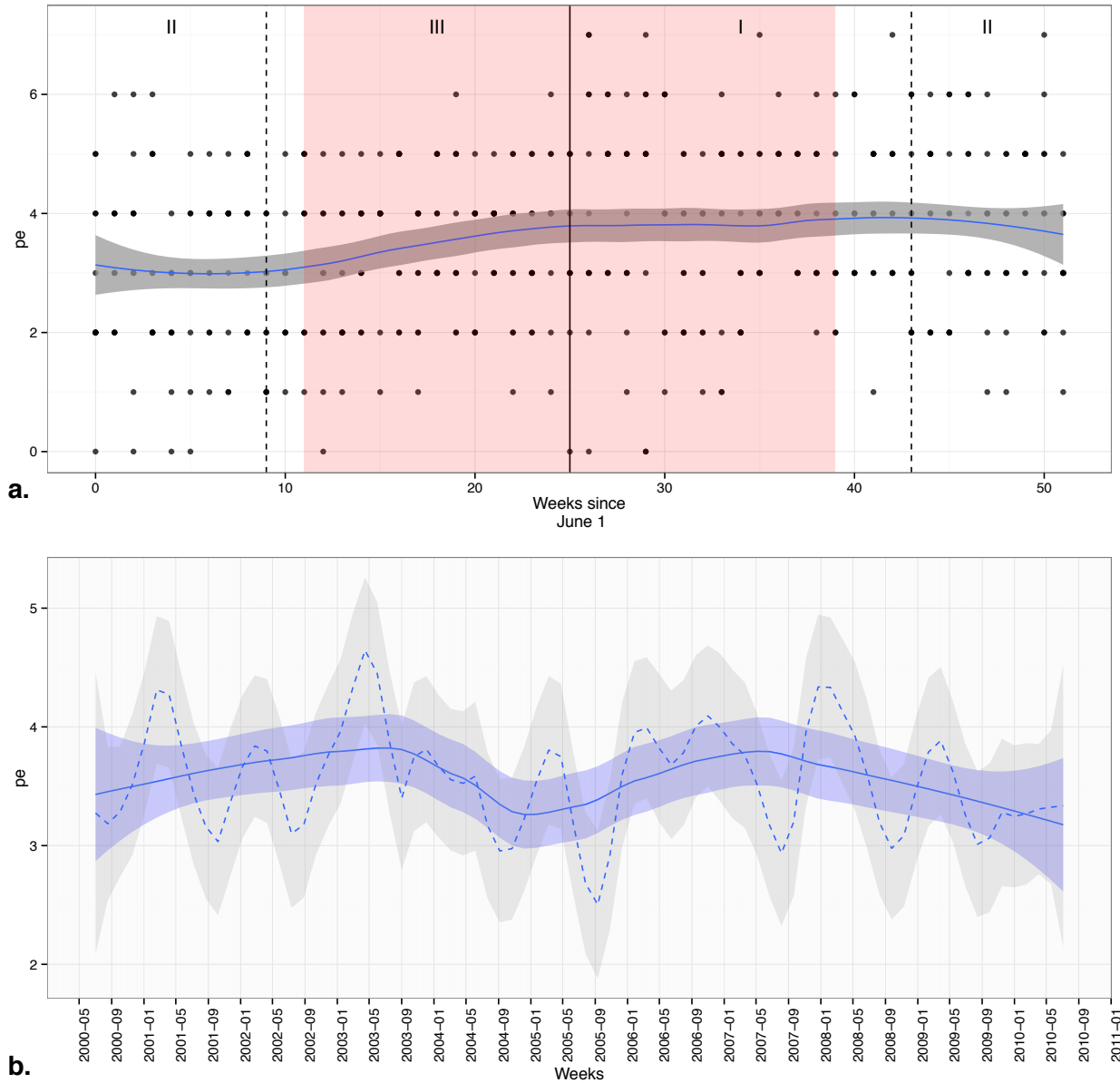
Figure S14: Seasonal (a) and long-term (b) trends of weekly precipitation events in Iquitos, Peru. In (a), annual trimesters (demarcated by dashed vertical lines) and the dengue season (red shaded area) are indicated. The blue line is the loess smoothed response with standard error, \alpha = 0.5 . In (b), solid line is the loess smoothed response with standard error ( \alpha = 0.5 , blue envelope). The dashed line is for \alpha = 0.1 with standard error (grey envelope, See Methods).
