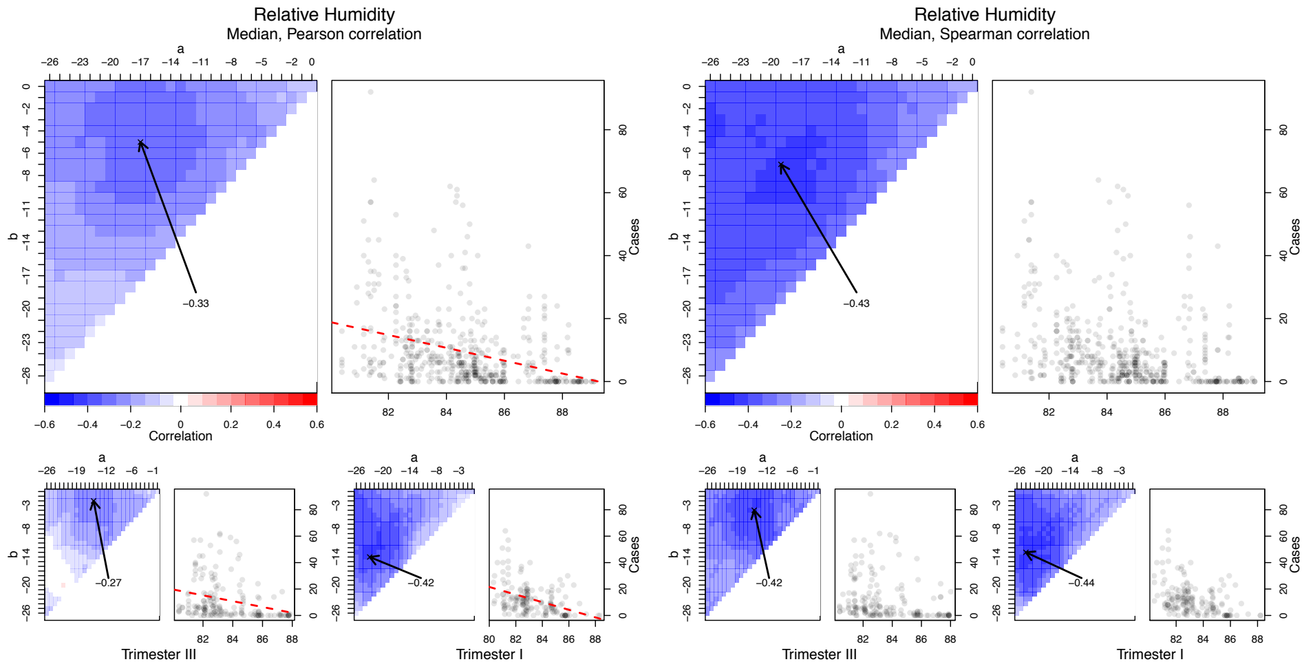
Figure S17: CCM and scatterplot at lag of highest |r| in Spearman and Pearson correlations for the whole year (large panels) and trimesters I and III.
