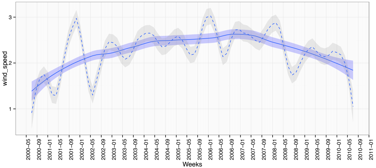
Figure S18: Seasonal (a) and long-term (b) trends of wind speed in Iquitos, Peru. In (a), annual trimesters (demarcated by dashed vertical lines) and the dengue season (red shaded area) are indicated. The blue line is the loess smoothed response with standard error, \alpha = 0.5 . In (b), solid line is the loess smoothed response with standard error ( \alpha = 0.5 , blue envelope). The dashed line is for \alpha = 0.1 with standard error (grey envelope, See Methods).
