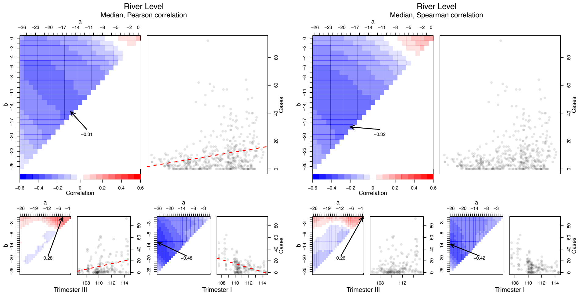
Figure S21: CCM and scatterplot at lag of highest |r| in Spearman and Pearson correlations for the whole year (large panels) and trimesters I and III.
