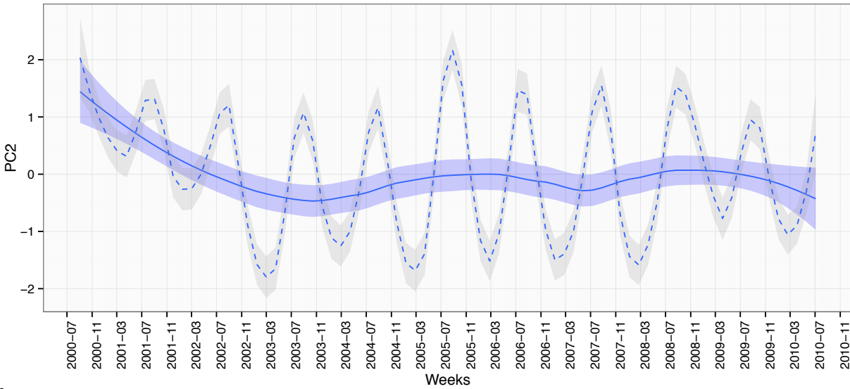
Figure S24: Seasonal (a) and long-term (b) trends of PC2 in Iquitos, Peru. In (a), annual trimesters (demarcated by dashed vertical lines) and the dengue season (red shaded area) are indicated. The blue line is the loess smoothed response with standard error, \alpha = 0.5 . In (b), solid line is the loess smoothed response with standard error ( \alpha = 0.5 , blue envelope). The dashed line is for \alpha = 0.1 with standard error (grey envelope, See Methods).
