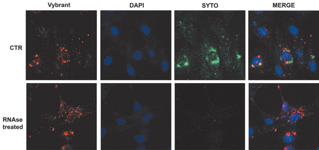
SUPPLEMENTARY FIG. S2. Specificity of RNA staining by RNase treatment of MSC-EVs. Double-labeled MSC-EVs treated or not with RNase were incubated with PTECs for 24 h. Vybrant ( red ) indicates the stained membrane of MSC-EVs and SYTO ( green ) indicates stained RNA derived from MSC-EVs. Nuclei stained by DAPI are blue . Three experiments were performed with similar results using MSC-EVs derived from different MSCs. Original magnification: \times 630 . CTR, control group.
