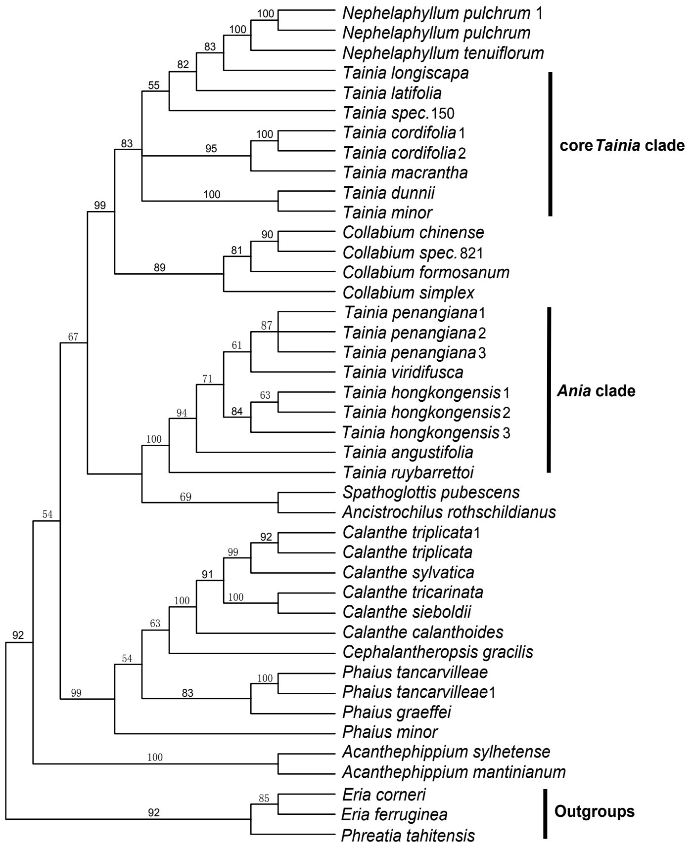
Fig. S1. Strict consensus tree of 3 equally parsimonious trees inferred using nr DNA ITS dataset to show the placement of Ania and the core Tainia . Bootstrap values are indicated above.
