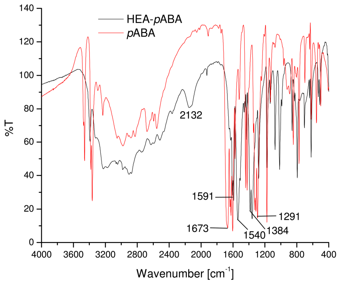
Figure S2. FT-IR spectra of HEA- p ABA (black) and p ABA (red).
