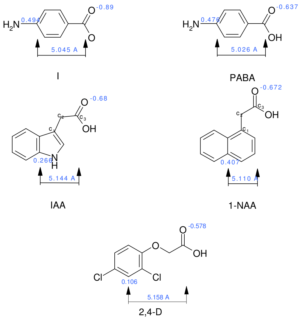
Figure S3. Optimal distance calculation for HEA- p ABA, p ABA and classical auxin molecules (IAA, 1-NAA, 2,4-D).
