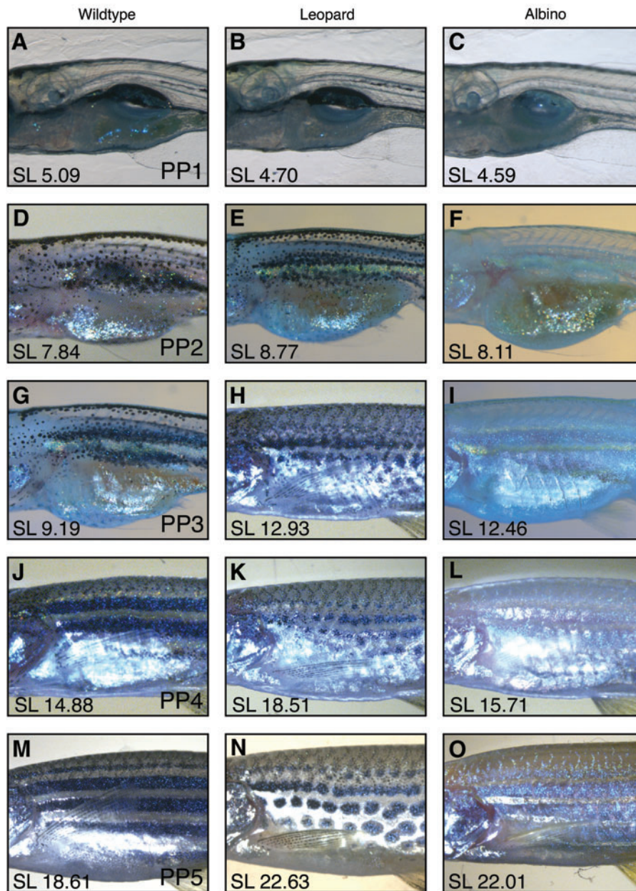
SUPPLEMENTARY FIG. S1. Pigment differences vary by stage as well as between fish of differing genotypes. Leopard mutants ( cx41.8 sl ) and albino mutant fish ( slc45a2 b4 ) were stage matched by standard length (SL) to appropriate wildtype fish. Wildtype fish PP1–5 ( A , D , G , J , M ), leopard pigmented fish ( B , E , H , K , N ), and albino fish ( C , F , I , L , O ) show different development of pigment pattern.
