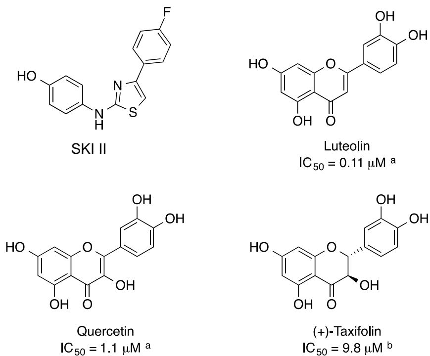
Figure S4. Structure of SKI II and some flavonoids which are known inhibitors of CB5R. Reported inhibitory activity ( IC_{50} ) for flavonoids is included ( a Çelik, H., Kosar, M. (2012) Chem. Biol. Int. 197 , 103-109. b Çelik, H., Kosar, M., Arinç, E. (2013) Toxicology 308 , 34-40).
