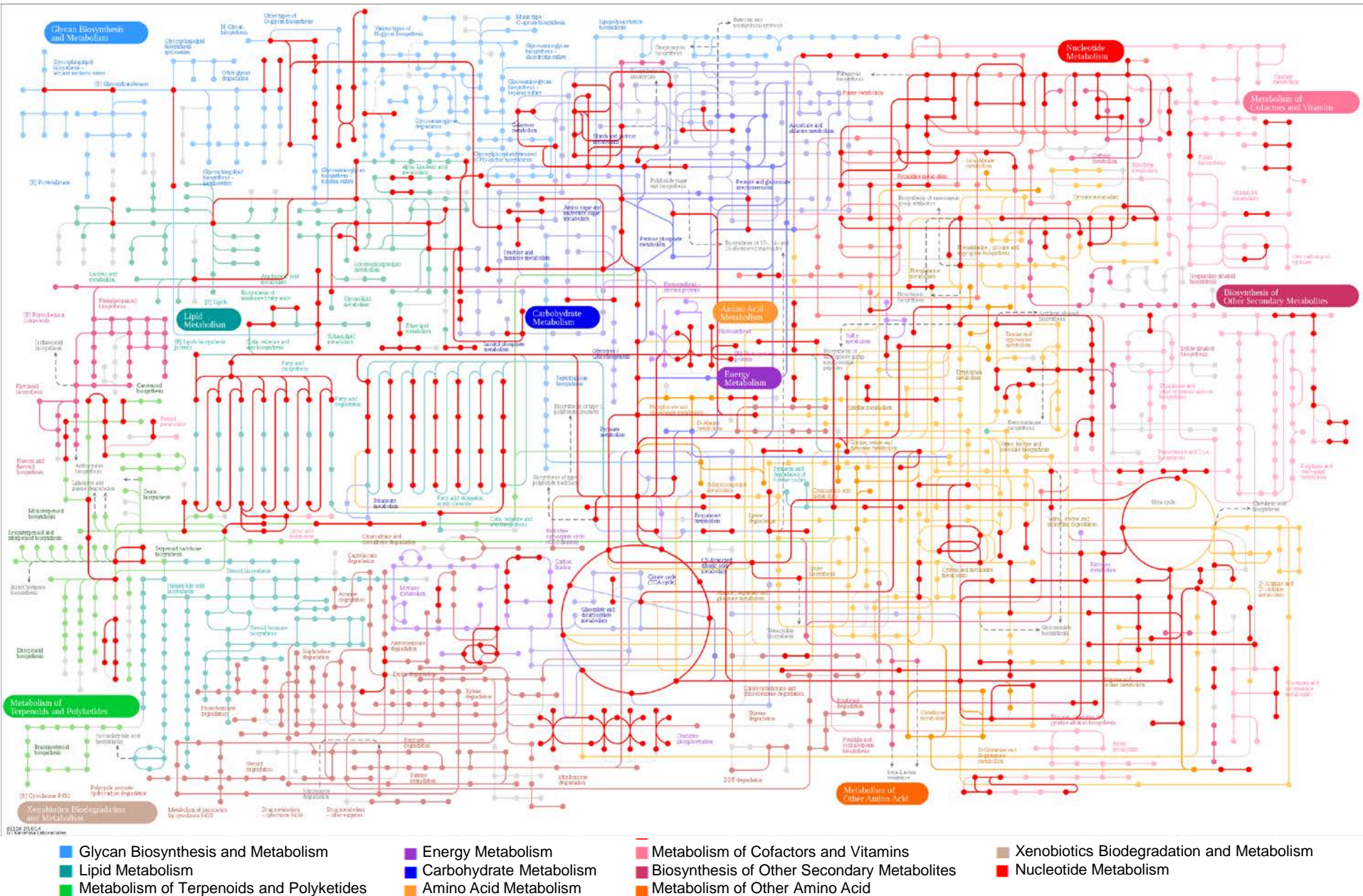
Fig. S6. KEGG pathway analysis of H. pluvialis . Cysts (B)
