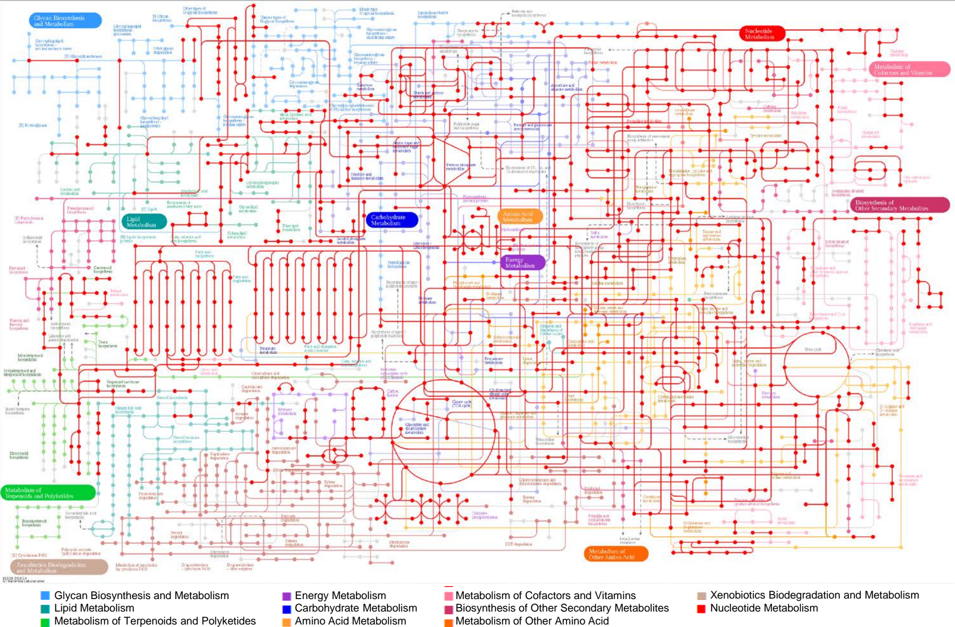
Fig. 5. Kyoto Encyclopedia of Genes and Genomes (KEGG) pathway analysis of H. pluvialis transcripts.
