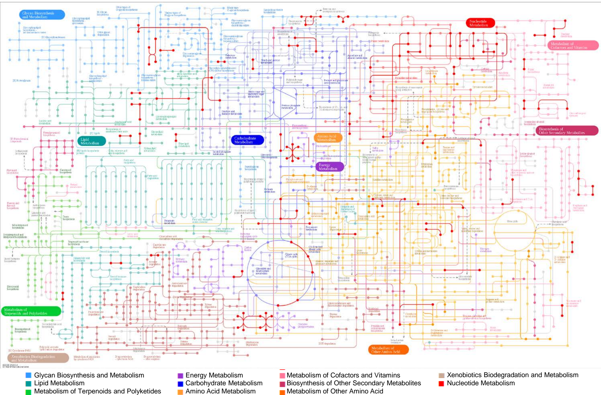
Fig. S6. KEGG pathway analysis of H. pluvialis . Macrozooids (A)
