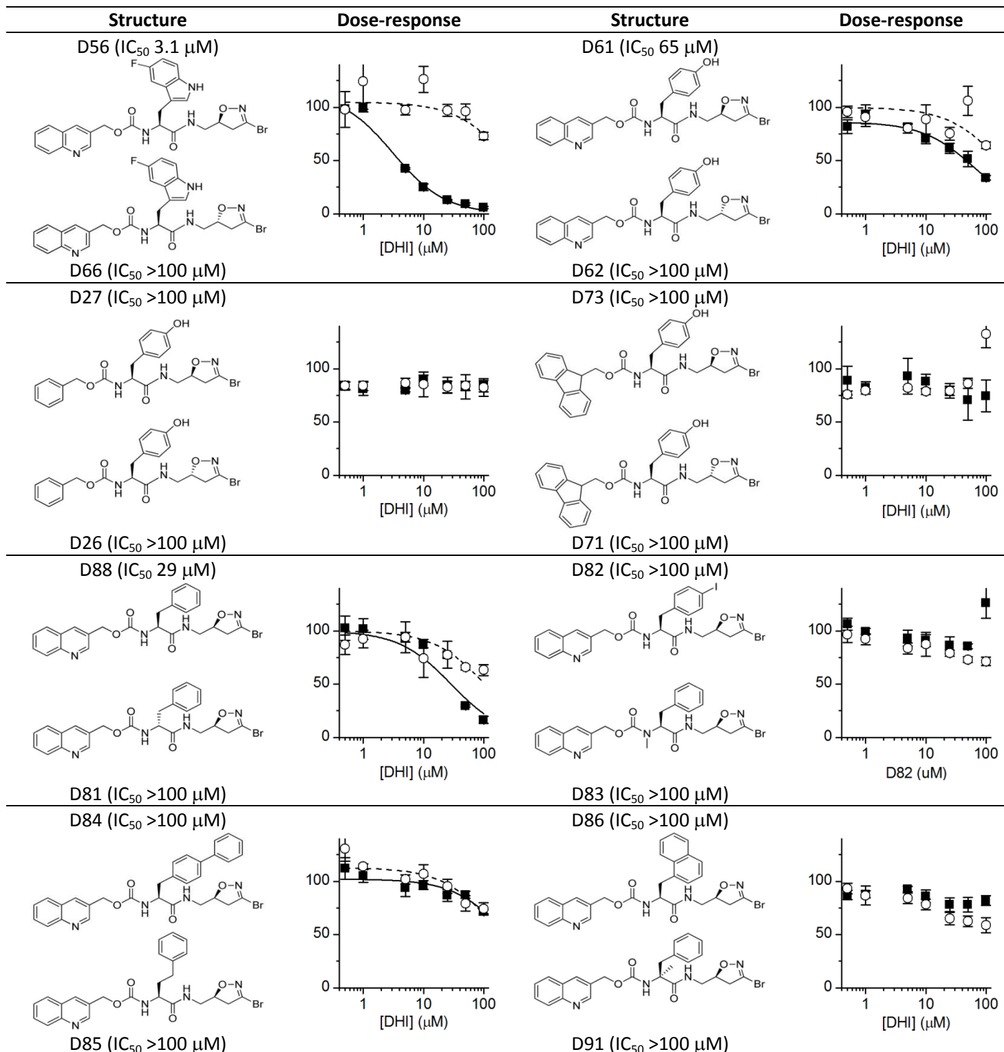
Supplementary Table 3. Graphical comparison of AgTG3 IC 50 for 27 dihydroisoxazole inhibitors
