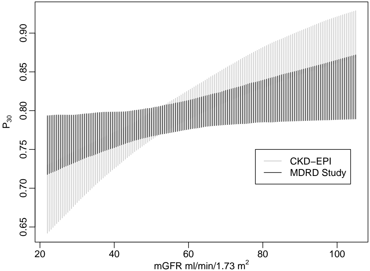
Figure S8: P 30 (99.6% CI) of the CKD-EPI and the MDRD Study equation across levels of measured GFR. Bars represent simulated (2000 simulations for each 1.0 ml/min/1.73 m 2 ) confidence intervals of the P 30 of the CKD-EPI (grey) and the MDRD Study equation (black) plotted against measured GFR. Outliers were excluded by only including mGFR values lying in 2.5%-97.5% of the distribution.
