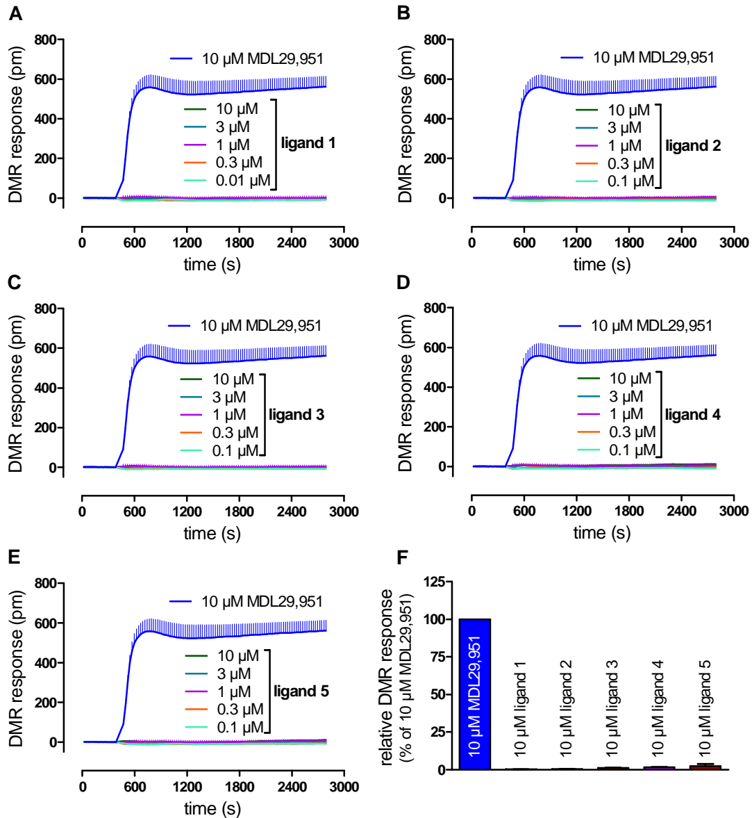
Fig. S12. MDL29,951 but not ASINEX ligands 1 to 5, display functional activity on rat GPR17. HEK-rGPR17 cells were stimulated with the indicated concentrations of ASINEX ligands 1-5 or the GPR17 agonist MDL29,951 as control and DMR was recorded over time. (A-E) Data are representative traces of mean + S.E., repeated independently twice; (F) Data are mean + S.E.M. of n= 2 independent experiments, each performed in triplicate.
