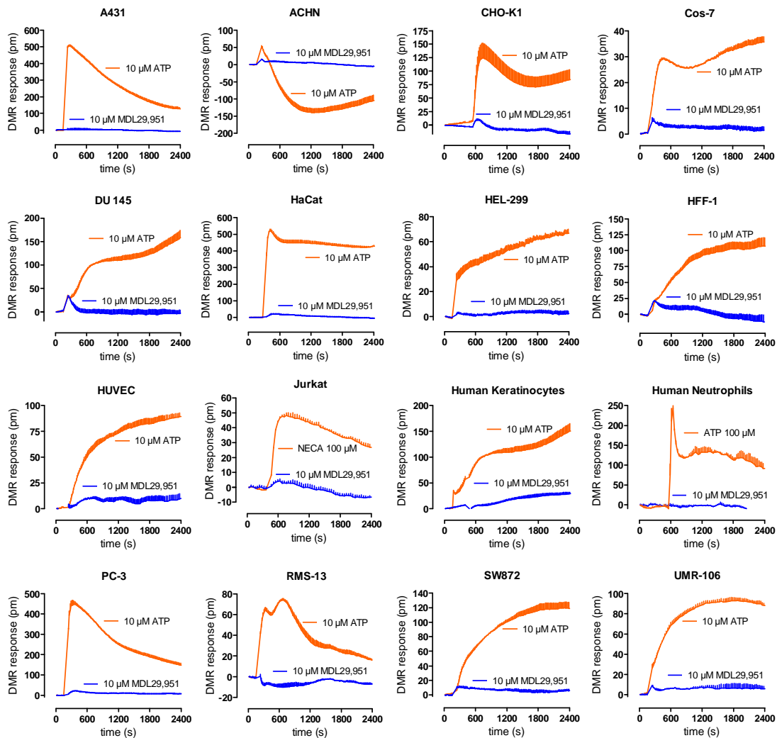
Fig. S16. MDL29,951 does not trigger cell activation across 16 distinct ATP-responsive immortalized and primary cell lines in a receptor panning approach. To trace functional endogenous receptors using ligands as a bait, cells were stimulated with the indicated concentrations of ATP (P2Y 1,2,4,6,11 agonist), the adenosine A 2a receptor agonist NECA, and GPR17 agonist MDL29,951 and label-free DMR responses were recorded over time. No endogenous MDL29,951-responsive receptor is detected. Data are mean + S.E. of representative DMR recordings repeated at least twice in triplicate.
