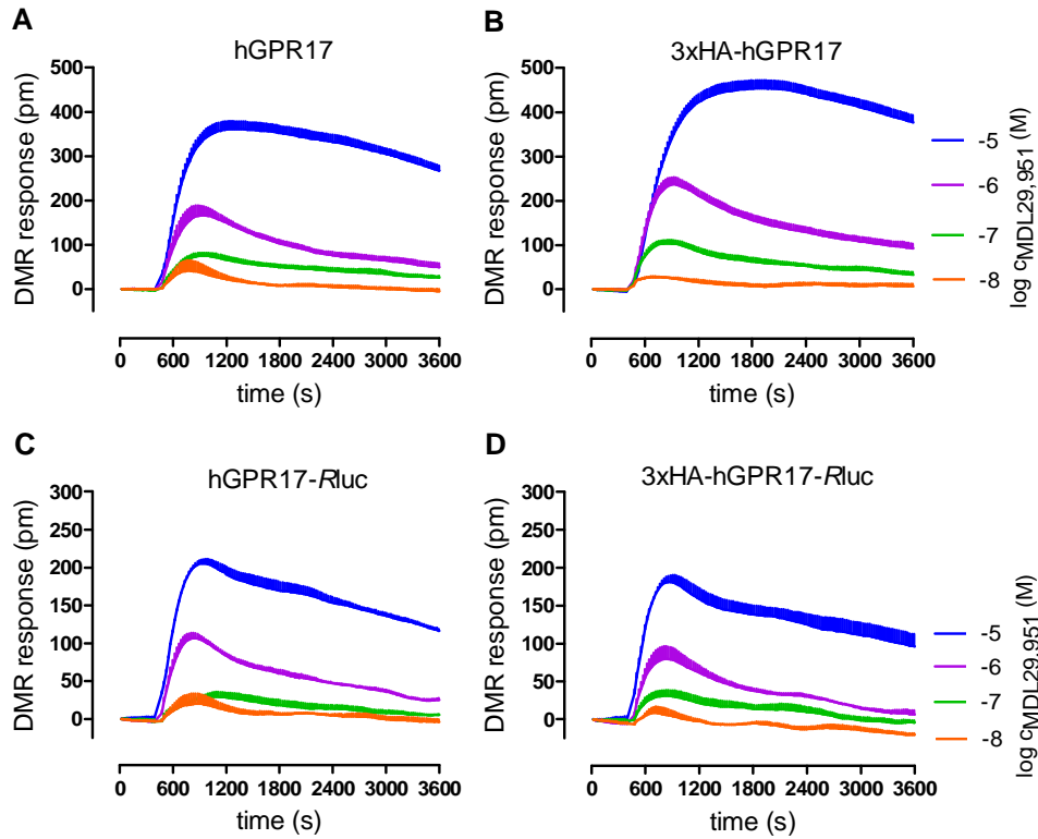
Fig. S22. Introduction of a triple HA tag at the N termini of hGPR17 and hGPR17-Rluc does not alter signaling capacity of the receptor constructs. HEK293 cells transfected to express the indicated untagged (A,C) and tagged (B,D) GPR17 constructs were stimulated with the GPR17 agonist MDL29,951 and DMR was recorded over time. Data are representative real-time DMR traces (mean + S.E.), repeated at least three times in triplicate with independent transfections.
