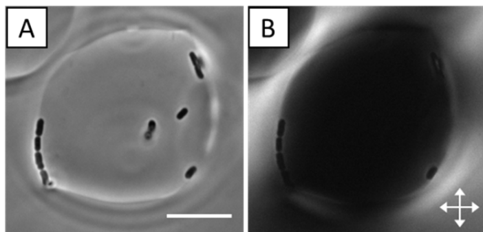
Figure S4. Trapping of non-motile cells at the boojum associated with an isotropic tactoid. (A) Bright field and (B) crossed polars micrographs of non-motile P. mirabilis cells adsorbed at the N-I interface of an isotropic tactoid. Scale bars are 10 \mu\text{m} .
