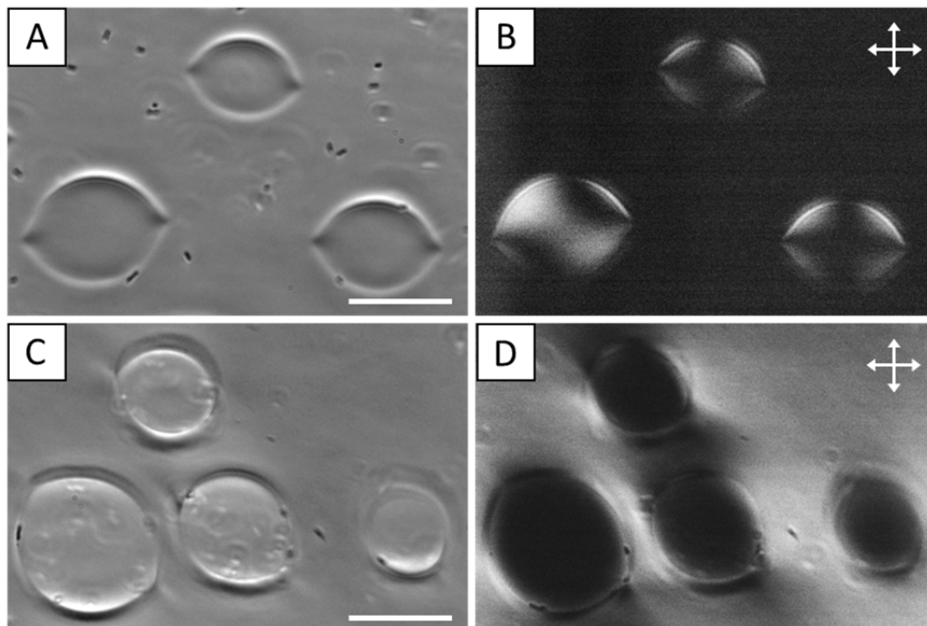
Figure S6. Temporal accumulation of motile bacteria at the interface of isotropic tactoids. ( A and B ) Bright field and crossed polars images, respectively of motile P. mirabilis cells dispersed in DSCG solution quenched to 33°C that contains nematic tactoids encompassed by isotropic phase solution. ( C and D ) Bright field and crossed polars images, respectively of motile P. mirabilis cells dispersed in DSCG solution heated to 30°C that contains isotropic tactoids surrounded by a continuous nematic phase. All images were obtained following 15 min of equilibration at the specified temperatures. Scale bars are 20 \mu\text{m} .
