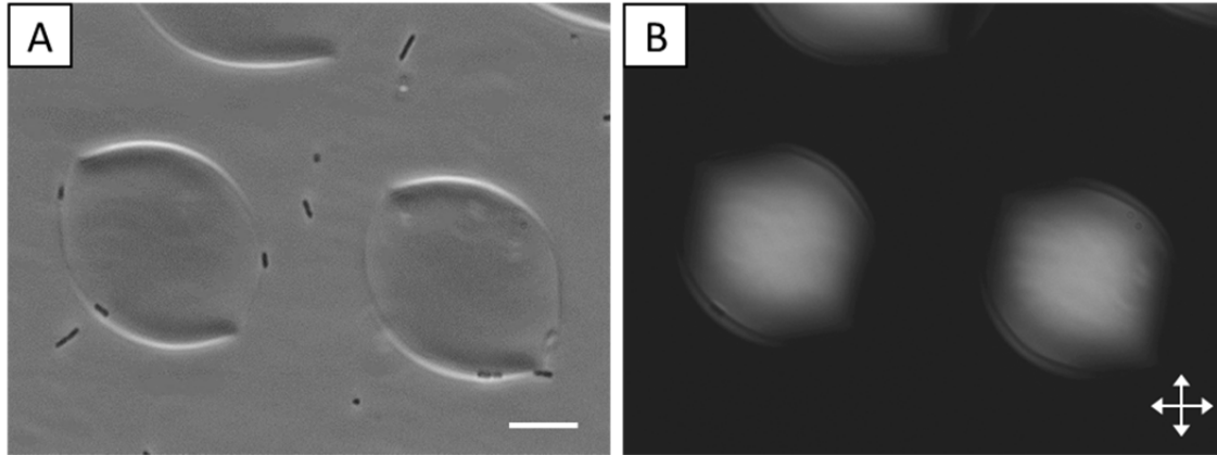
Figure S3. Orientations of non-motile bacteria adsorbed to nematic tactoids. (A) Bright field and (B) crossed polars images, respectively, of non-motile P. mirabilis cells adsorbed at the interface of nematic tactoids that formed on a glass substrate following cooling of an isotropic phase of DSCG (15 wt%) from 40°C to 33°C. The scale bar is 10 \mu\text{m} .
