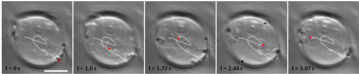
Figure S5. Escape of an adsorbed motile cell into the interior of an isotropic tactoid. Sequence of bright field micrographs that depicts the trajectory of a motile P. mirabilis cell, initially adsorbed to the interface of an isotropic tactoid, which escapes into the interior of the tactoid. The trajectory of the cell (indicated by a red dot) is depicted in the images. The random motion of the cell suggests that it is not adsorbed to the N-I interface. The scale bar is 10 \mu\text{m} .
