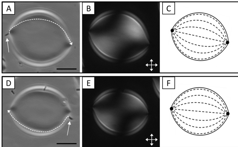
Figure S2. Additional examples of LC elasticity-induced guided motility of cells adsorbed to nematic tactoids. Two examples ( A–C and D–F ) of the motility of P. mirabilis cells adsorbed to the interface of nematic tactoids. ( A and D ) Bright field micrographs of nematic tactoids on which the trajectories of motile P. mirabilis cells (indicated by arrows) adsorbed to the N-I interface are indicated. ( B and E ) Corresponding crossed polars images. ( C and F ) Schematic representations of the LC director profiles of the tactoids in B and E , respectively. Scale bars are 10 \mu\text{m} .
