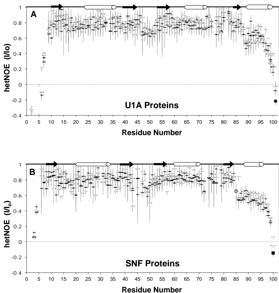
Figure S5. Backbone amide ^{15}\text{N} - \{^1\text{H}\} heteronuclear NOE data for U1A and SNF RRM1. (A) U1A RRM1 proteins: wild type U1A ●, U1A(F56Y) ■, U1A(Y13F) ○, U1A(Y13F/F56Y) □, U1A(Q54F) Δ, and in (B) SNF RRM1 proteins: wild type SNF ●, SNF(F53Y) ■, SNF(Y10F) ○, SNF(Y10F/F53Y) □. Secondary structural elements are shown above the panel for reference. Errors were determined from the propagation of baseplane noise. Larger errors occur in SNF regions of broadened exchange, particularly in loop 3 where the signal/noise is poor.
