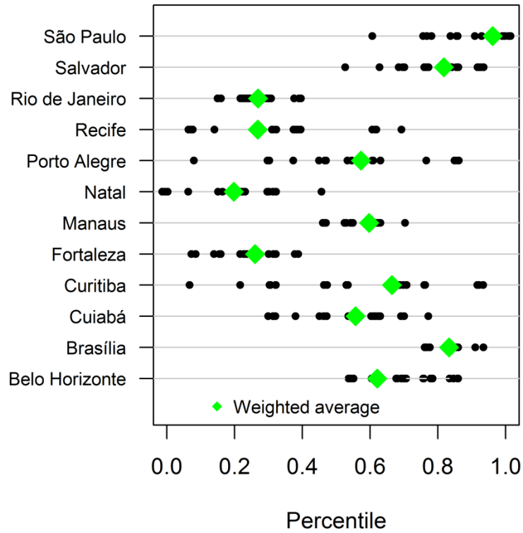
Figure S1, Percentile of 2014 weekly IR's on distributions of previous years. For each game city, the percentile of 2014 weeks 1 to 19 on the 2001-2013 distributions for the same weeks is shown (black) with some x-axis random variation to see the individual points. The average percentile weighted by the week number is shown in green (P2014).
