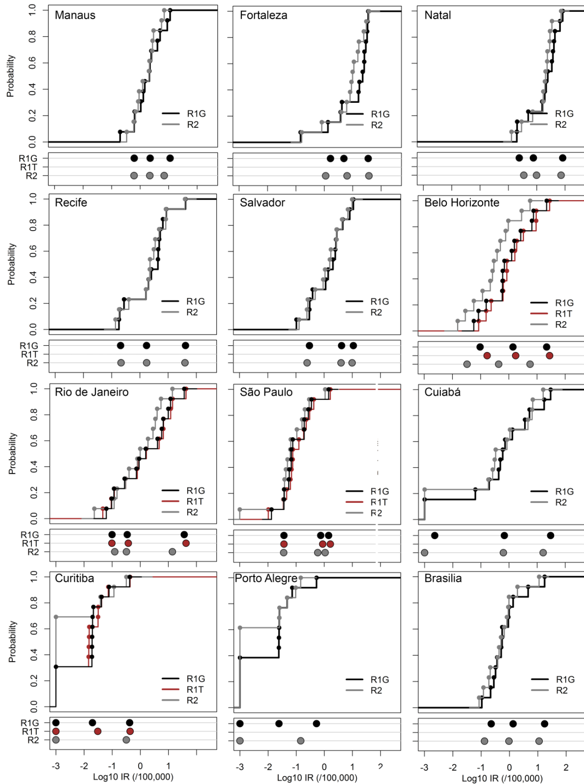
Figure S2. Probability distribution of average log 10 incidence rates (/100,000) in game cities of the 2001-2013 period during the weeks of World Cup round one (teams: R1T and tourists: R1G) and round two (R2) of the 2014 World Cup. For each period, the 10 th percentile (P10), P2014 and maximum are indicated.
