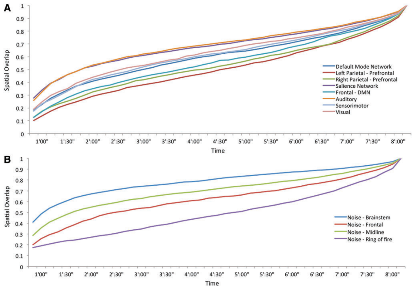
SUPPLEMENTARY FIG. S3. Network stability of the group mean of 84 subjects from the dual regression analyses, (A) eight brain network components and (B) four noise components, with respect to time of acquisition.
