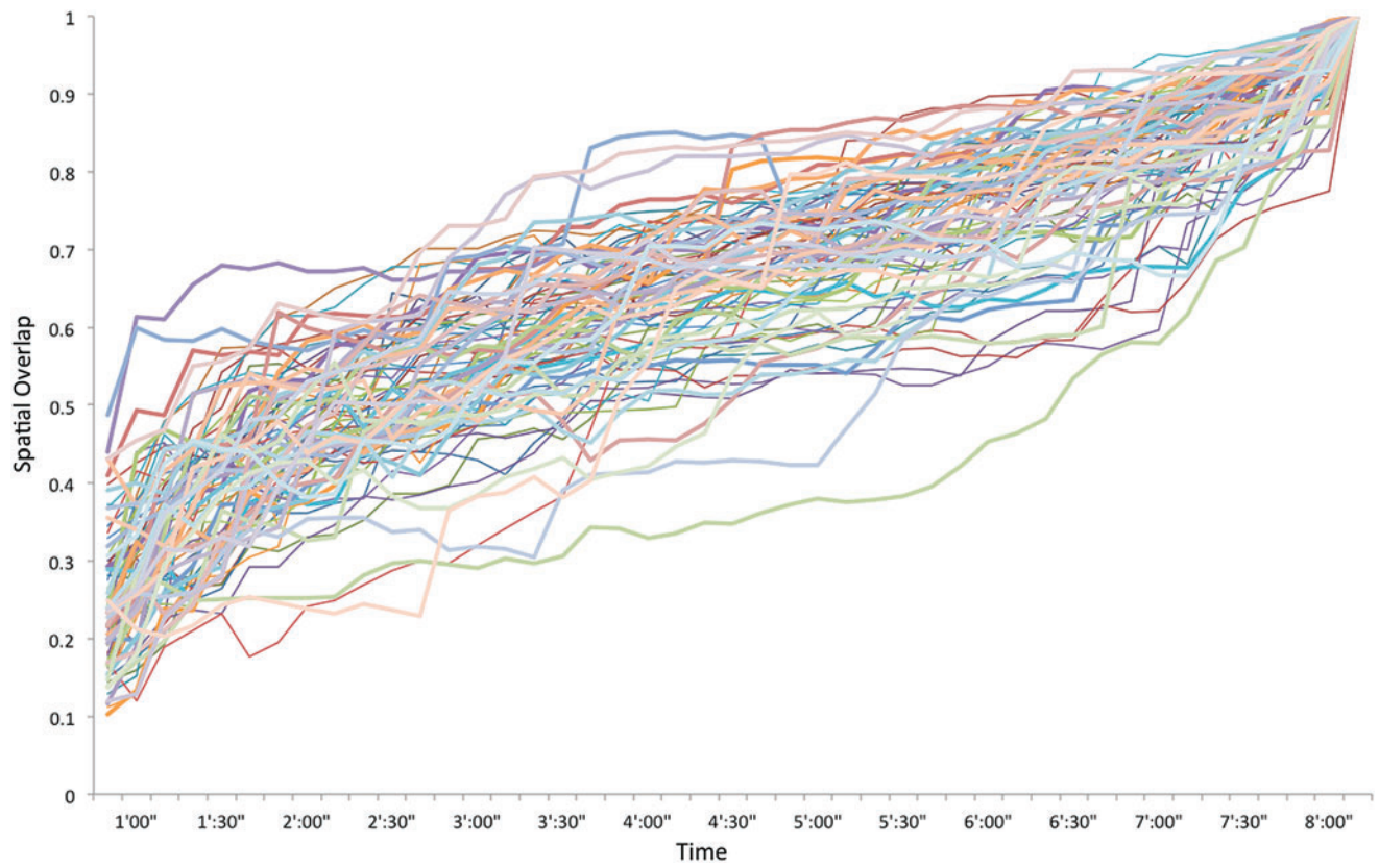
SUPPLEMENTARY FIG. S5. Network stability of the DMN in 84 subjects from the dual regression analyses with respect to time of acquisition.
