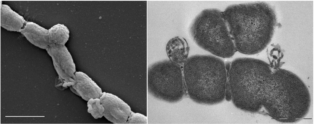
Figure S1. SEM and TEM images (left and right panels, respectively) of TolB-deficient mutant cells grown as described in the legend to Figure 3A. Bars: 1 \mu\text{m} (left panel) or 0.5 \mu\text{m} (right panel).
