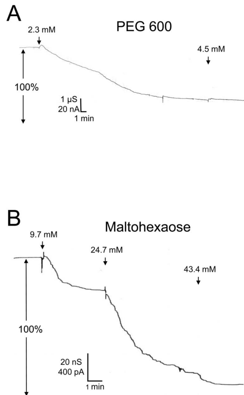
Figure 4. Titration of the P66-induced membrane conductance with PEG 600 (A) and maltohexaose (B). The membrane was formed with PC/ n -decane. The aqueous phase contained \sim 100 \text{ ng ml}^{-1} P66, 1 M KCl and respective nonelectrolytes in the concentration as indicated; temperature = 20°C; applied voltage = 20 mV. doi:10.1371/journal.pone.0078272.g004
