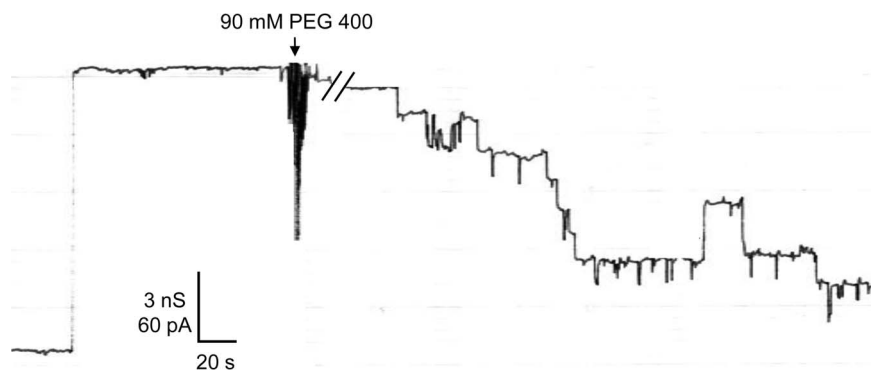
Figure 5. PEG 400-induced blockage of P66 on the single-channel level. Small amounts of highly diluted P66 (1:1,000 in 1% Genapol) was added to both sides of a diphtanoyl PC membrane. After reconstitution of one single 11 nS P66 unit, 90 mM PEG 400 was added to both sides of the membrane. The P66 conductance was blocked stepwise exhibiting subconductance steps of approximately 1.5 nS; temperature = 20°C; applied voltage = 20 mV.
