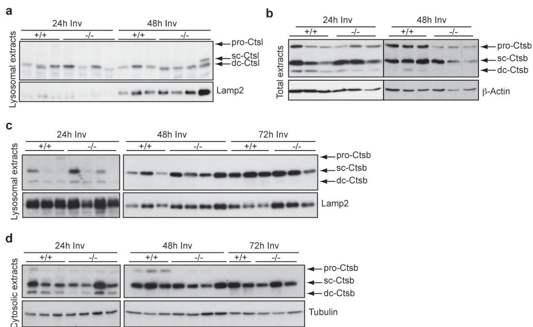
Supplementary figure 3. Cathepsin B is unaffected in the p55\alpha^{-}/p50\alpha^{-} mice. (a) Western blot analysis showing no differences in the expression of cathepsin L (Ctsl) in the lysosomal fraction of glands of p55\alpha^{-}/p50\alpha^{-} mice when compared to controls. Total (b) , lysosomal (c) and cytosolic (d) fractions display no major differences in the levels of cathepsin B (Ctsb) in the glands of p55\alpha^{-}/p50\alpha^{-} mice when compared to controls at the indicated hours of involution. -/-, p55\alpha^{-}/p50\alpha^{-} glands; +/+, p55\alpha^{+/+}/p50\alpha^{+/+} glands. Lamp2 and Tubulin are shown as lysosomal and cytosolic markers, respectively; \beta -Actin is shown as loading control for the total extracts.
