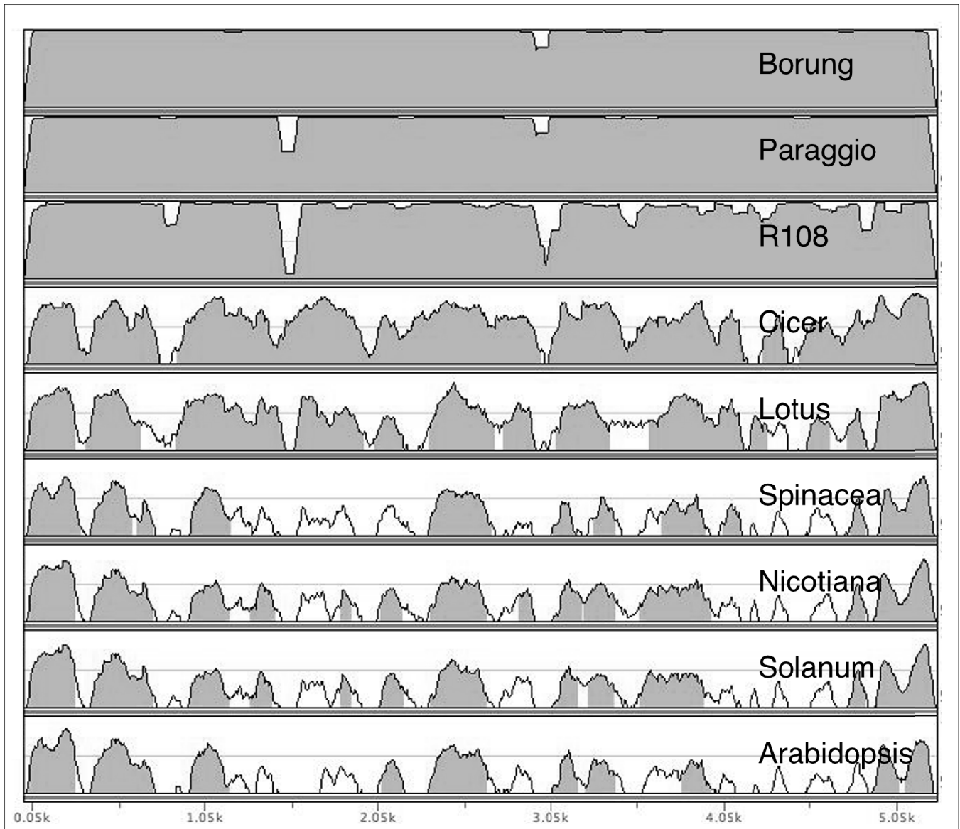
Supplementary Figure S3. The ycf1 mVISTA similarity plot of Borung, Paraggio, R108 and angiosperm species Cicer arietinum (NC_011163), Lotus japonicus (NC_002694), Nicotiana tabacum (NC_001879), Solanum lycopersicum (NC_007898), Spinacea oleracea (NC_002282) and Arabidopsis thaliana (NC_000932) compared to the M. truncatula 2HA line. The window is 100 bp, the consensus width is 100 bp and the consensus identity is 70%.
