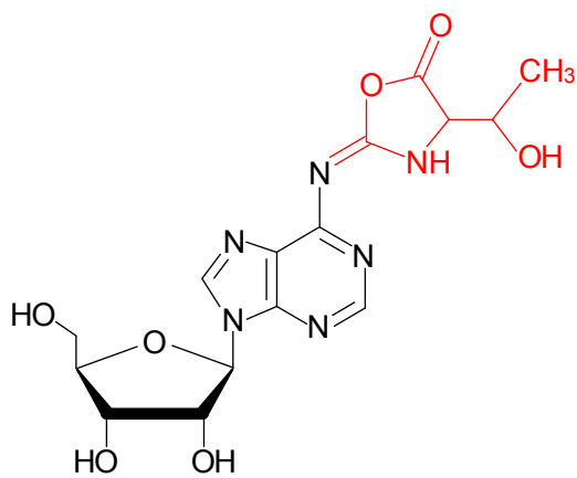
Cyclic- N 6 -threonylcarbamoyladenine ( ct 6 A)
