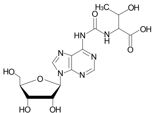
N 6 -threonylcarbamoyladenine ( t 6 A)
