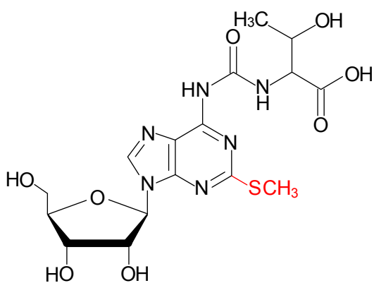
2-methylthio- N 6 -threonylcarbamoyladenine ( ms 2 t 6 A)
