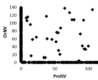
Fig. S1. Gene parity plots comparing ORF content and order of PmNV with (A) HzNV-1 and (B) OrNV. ORFs present in only one of the compared genomes appear on the axis corresponding to the virus in which they are present.
