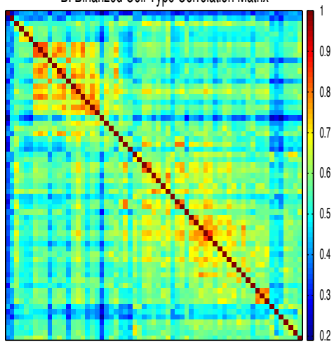
B. Binarized Cell Type Correlation Matrix
