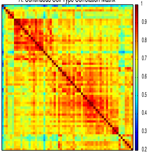
A. Continuous Cell Type Correlation Matrix
