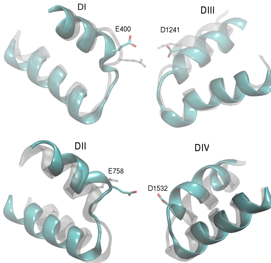
Figure 1: Snapshot comparing the pore domain of our Nav1.4 model with that of Chen et al. [75].
