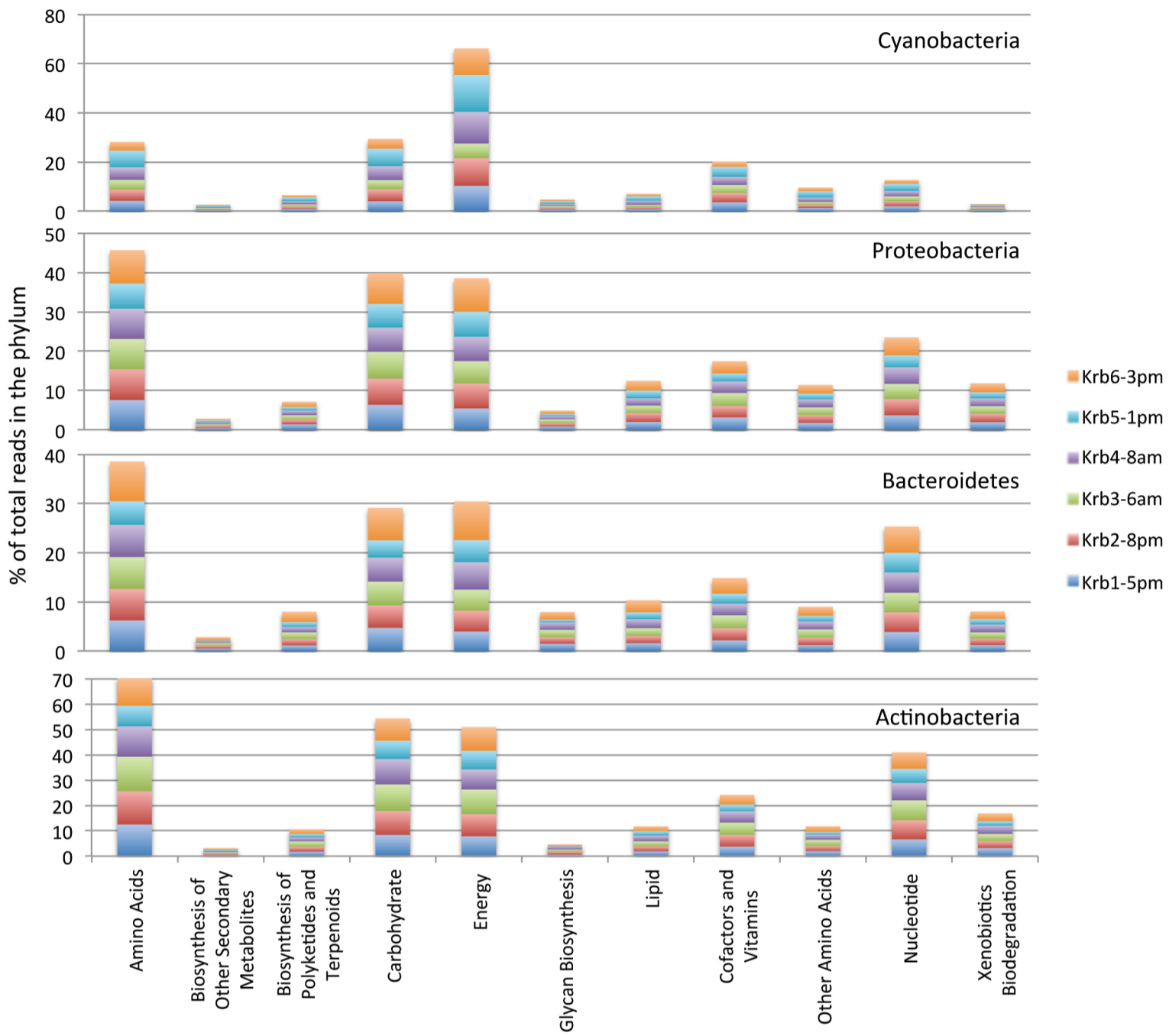
Supplementary Figure 5 Bar graph showing the distribution of transcripts from KEGG metabolism pathways
