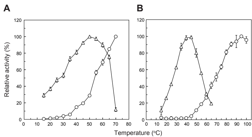
FIGURE S2. Temperature dependence of Pyr2C reductase (A) and T3LHyp dehydratase activities (B). Circle, each enzyme from T. litoralis (TILhpI and TILhpH); triangle, each enzyme from A. brasilense (AbLhpI and AbLhpH). Values are the means \pm SD, n = 3.
