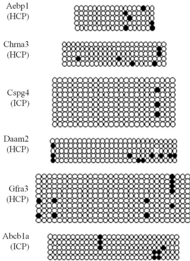
SUPPLEMENTARY FIG. S7. Methylation status in the gastrulating epiblast (E7). Circles represent CpG nucleotides either methylated ( closed ) or unmethylated ( open ).
