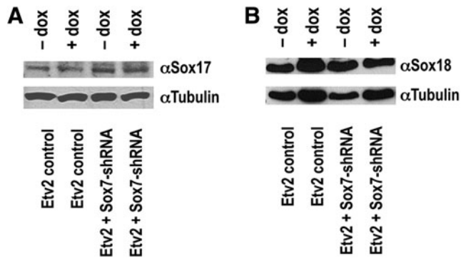
SUPPLEMENTARY FIG. S2. EBs were prepared using ETV2 over-expressing mES cells containing lentivirus constitutively expressing shRNA for Sox7 or control. Dox was added for 72 h (days 3–6) and EBs cultured for 6 days. Western blot analysis in EBs collected on day 6. Closely related Sox-F family member SOX17 ( A ) or SOX18 ( B ) protein levels were analyzed by western analysis. No decrease in SOX17 or SOX18 was detected, indicating knockdown specificity of the Sox7 shRNA to Sox7 .
