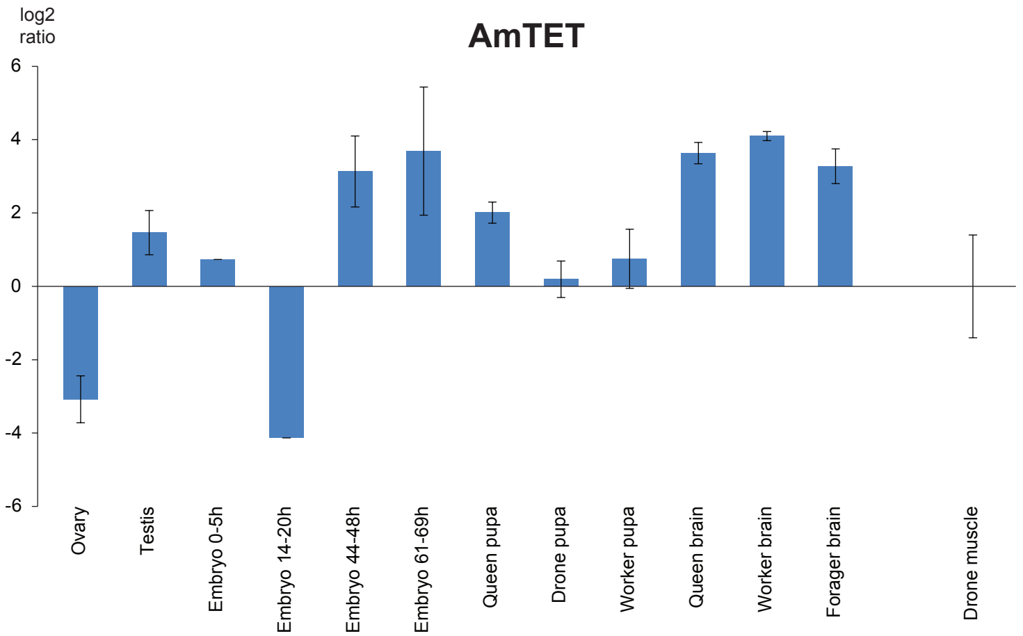
Figure S3. qPCR analysis of AmTET and AMDNMT3 expression in various honey bee samples. See material and methods for more details.
