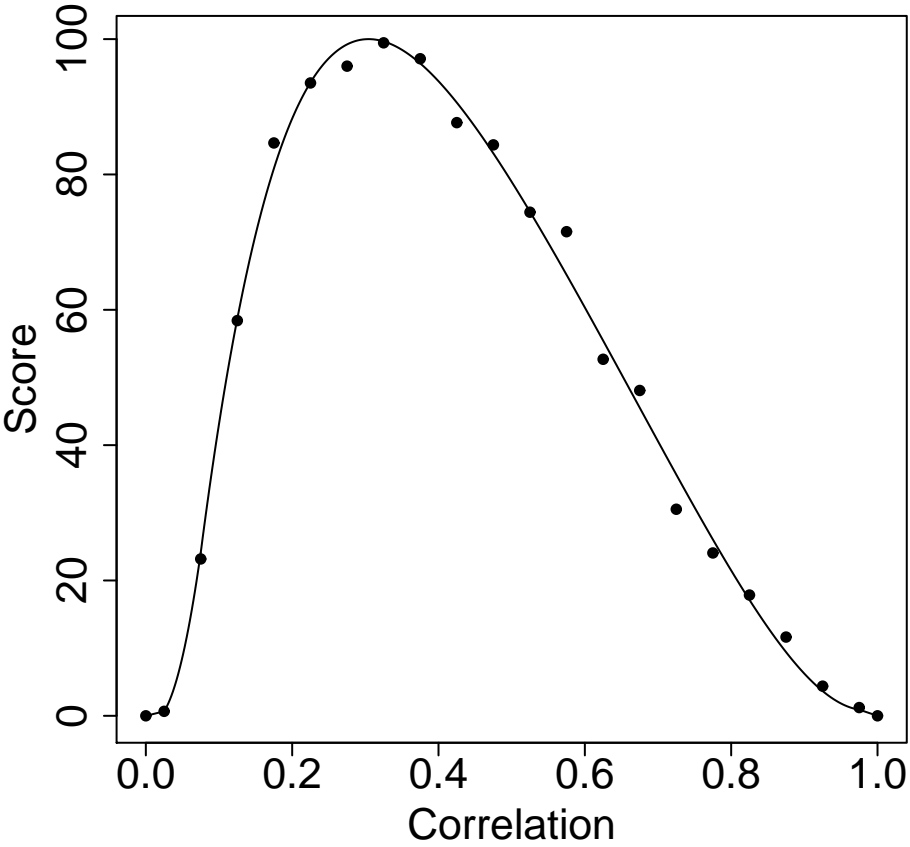
Multiplicative Correlation Metric
