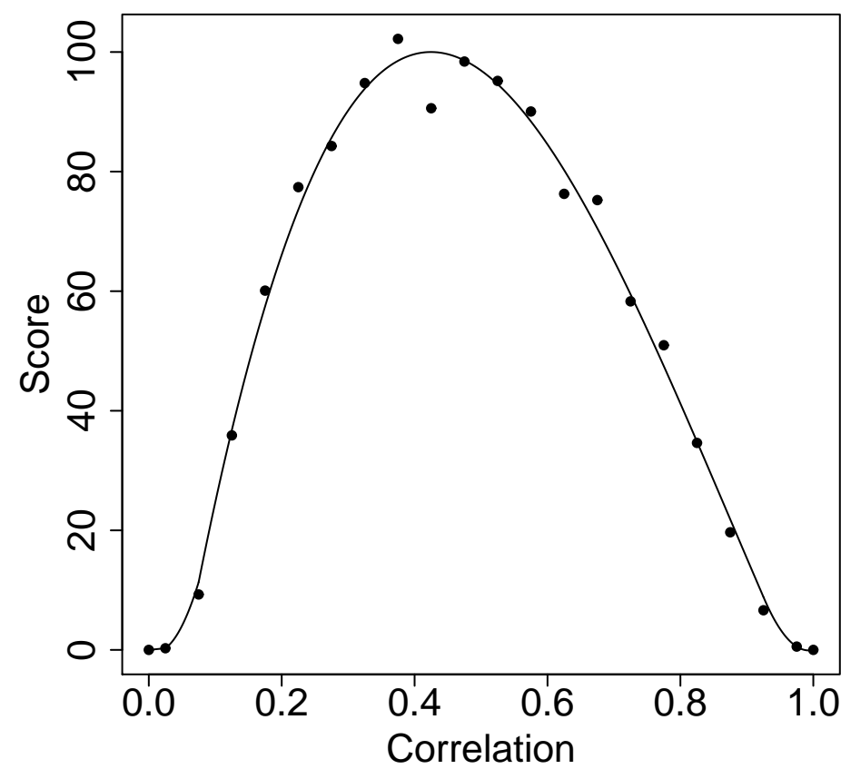
Recessive Correlation Metric
