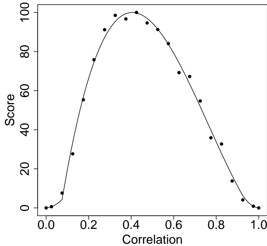
Dominant Correlation Metric
