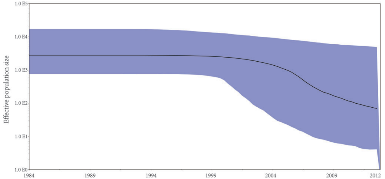
SUPPLEMENTARY FIG. S1. Demographic history of the expansion of HIV-1 subtype B' lineages in China. Bayesian skyline plot was estimated to reconstruct the demographic history of subtype B' in China using BEAST 1.4. The x -axis is the time in units of years and the y -axis is equal to the effective population size. The thick solid line is the mean estimates and the 95% HPD credible region is shown by blue areas.
