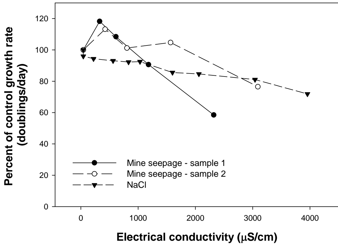
Figure S3 Response of Chlorella sp. growth rate to Mine seepage (samples 1 and 2) and NaCl, with concentrations expressed as Electrical Conductivity.
