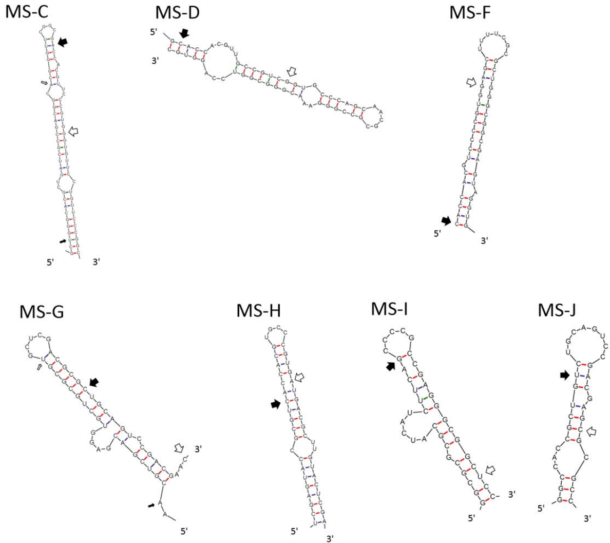
Figure S4. Predicted secondary structure for small RNAs of M. smegmatis .
