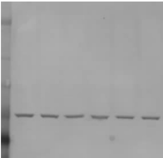
IB: GAPDH (NP40-Soluble)
