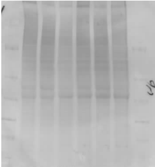
IB: Ubiquitin (NP40-Soluble)
