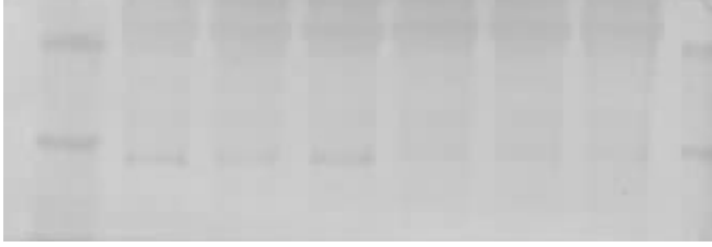
IB: V5 (NP40-Soluble)
