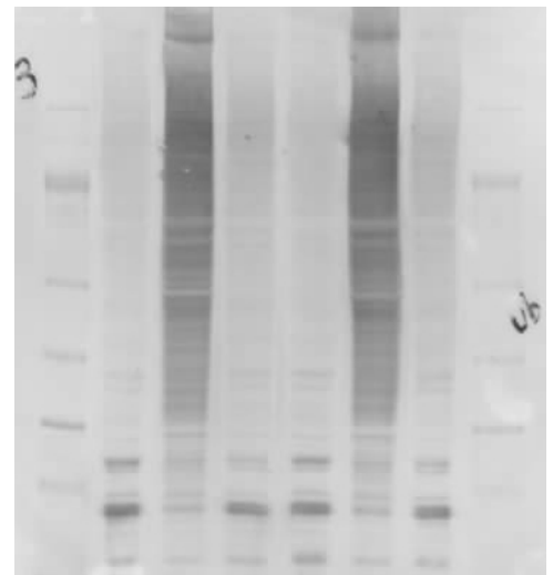
IB: Ubiquitin (NP40-Insoluble)
