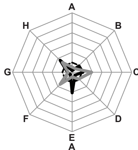
1% of Voxels
