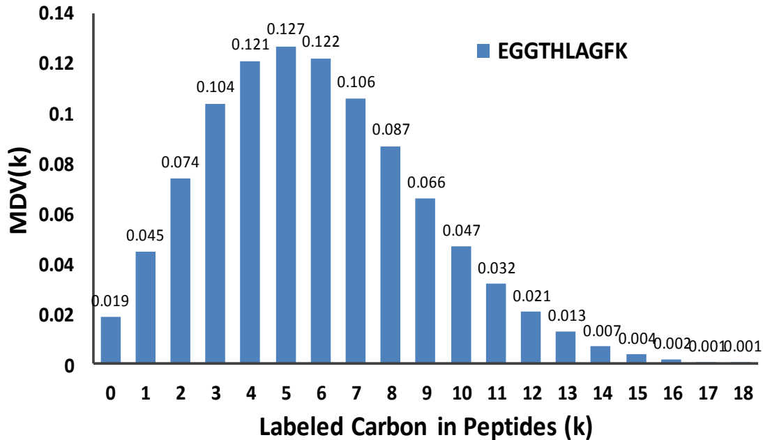
Figure S7. Peptide labeling profile for peptide based ^{13}\text{C} MFA obtained for D. vulgaris and M. maripaludis species in microbial community. Four 10 aminoacids peptides sequences and MDV's were plotted for (a) DDFEPVNEVK, (b) NPEITDEENK, (c) GTALSGDDVR and (d) EGGTHLAGFK.
